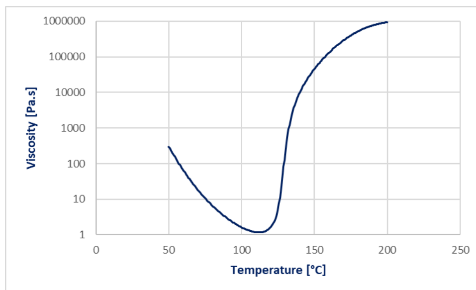
Figure 1 Rheology of AX-170MT
